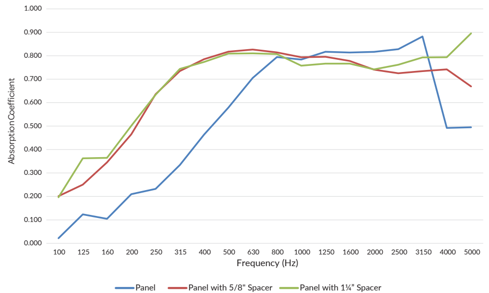
Absorption Spectrum of Tested Panels
