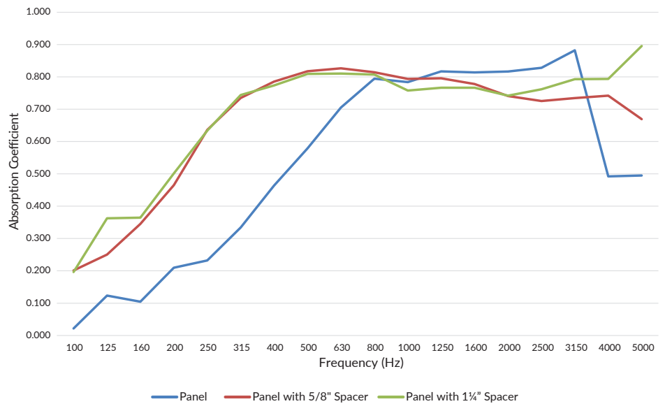
Absorption Spectrum of Tested Panels
